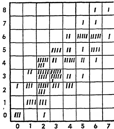
FIG. XIV. Scatter diagram. Correlation of approximately +0.8.
